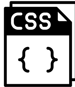
Advance CSS
