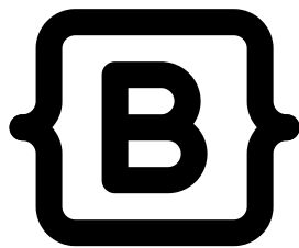
Bootstrap
