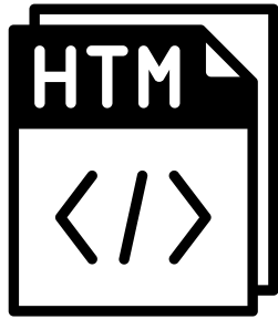
HTML - 5
